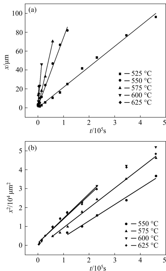
Fig. 7 Relationships of \text{TiAl}_3 layer thickness and annealing time at different annealing temperatures: (a) At chemical reaction-controlled growth stage; (b) At diffusion-controlled growth stage
