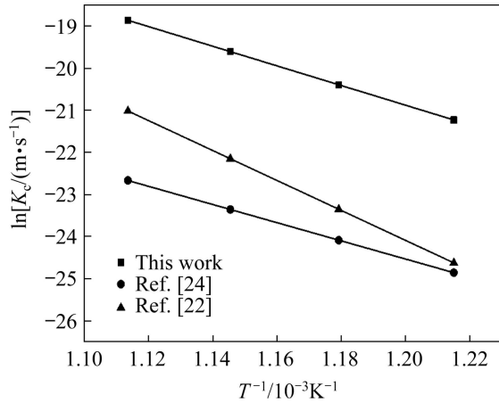
Fig. 10 Plot of \ln K_c versus T^{-1} for \text{TiAl}_3 layer obtained by different researchers
