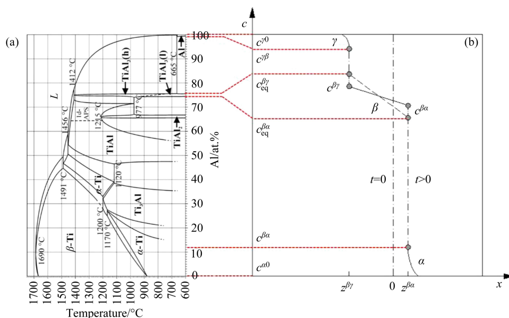
Fig. 9 Ti–Al binary alloy phase diagram [20] (a) and schematic diagram of Al concentration profile in \alpha , \beta and \gamma
