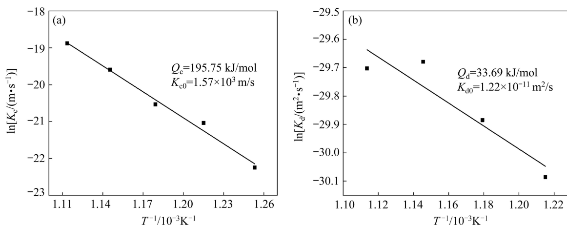
Fig. 8 Plot of \ln K_c versus T^{-1} for \text{TiAl}_3 layer at chemical reaction-controlled growth stage and plot of \ln K_d versus T^{-1} for \text{TiAl}_3 layer at diffusion-controlled growth stage
